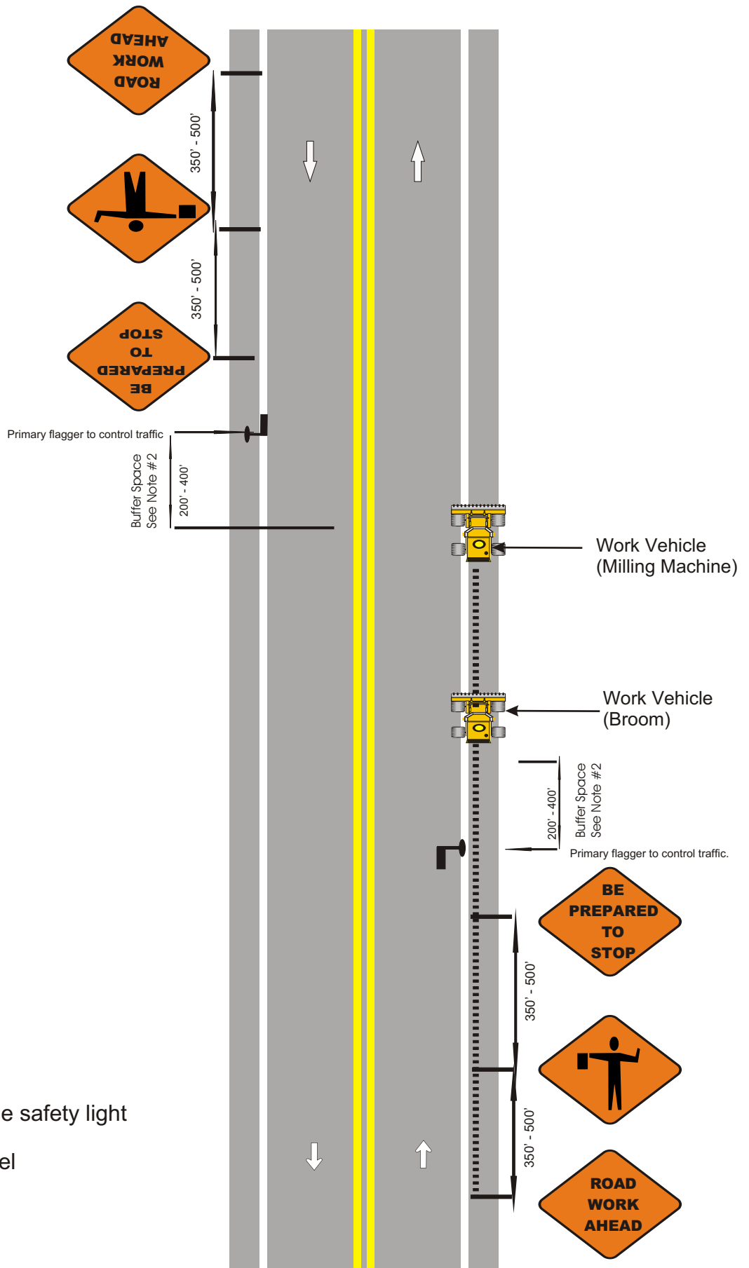
TWO LANE TWO WAY TRAFFIC CONTROL UTILIZING A MOVING FLAGGING OPERATION - SHOULDER OR EDGELINE RUMBLE STRIP CUTTING
